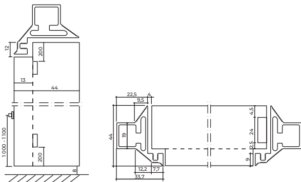
Frame SLIM TS
